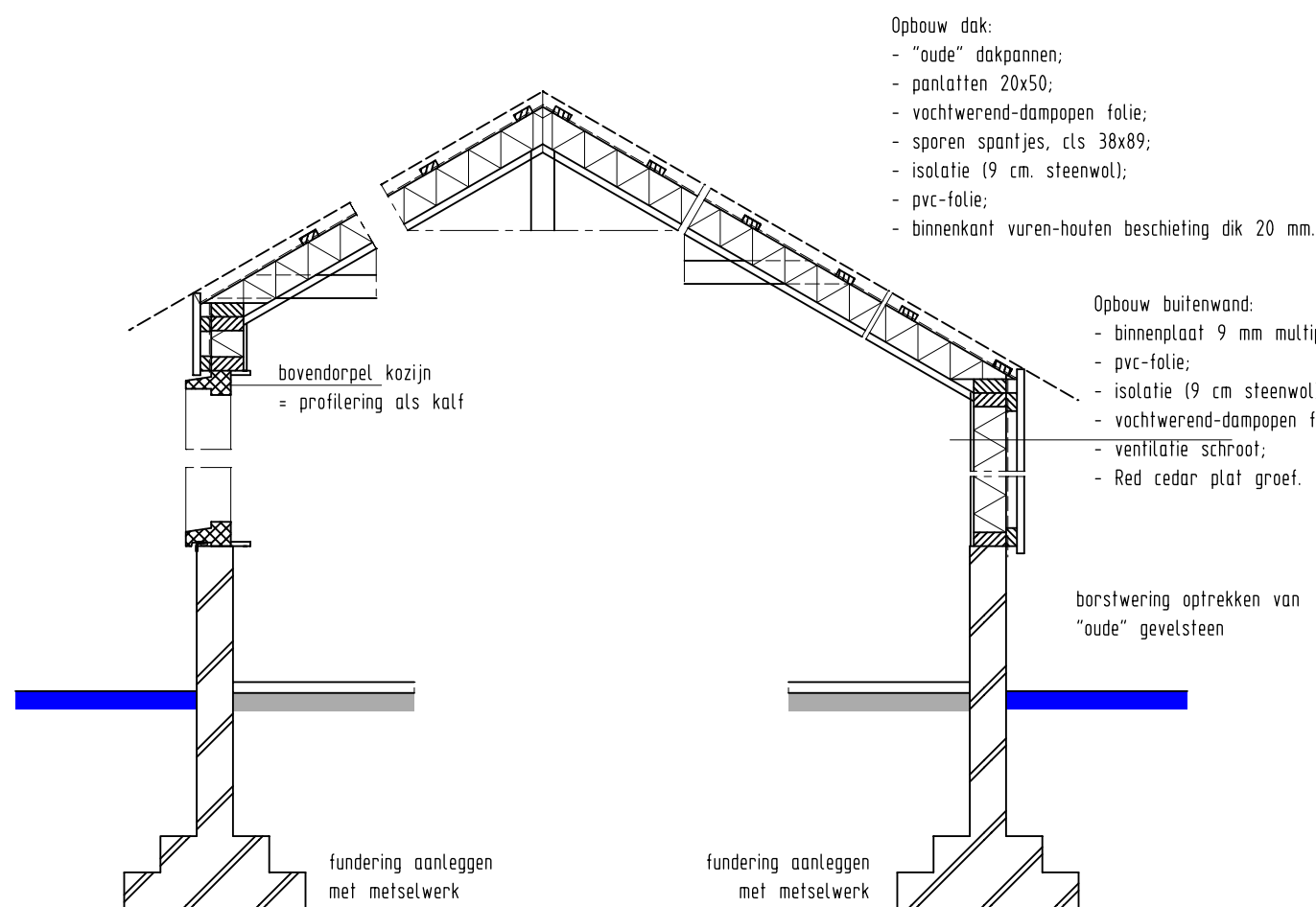
Details 1:20
